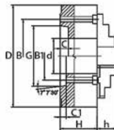
Back view Type A1 Bolt hole pattern
